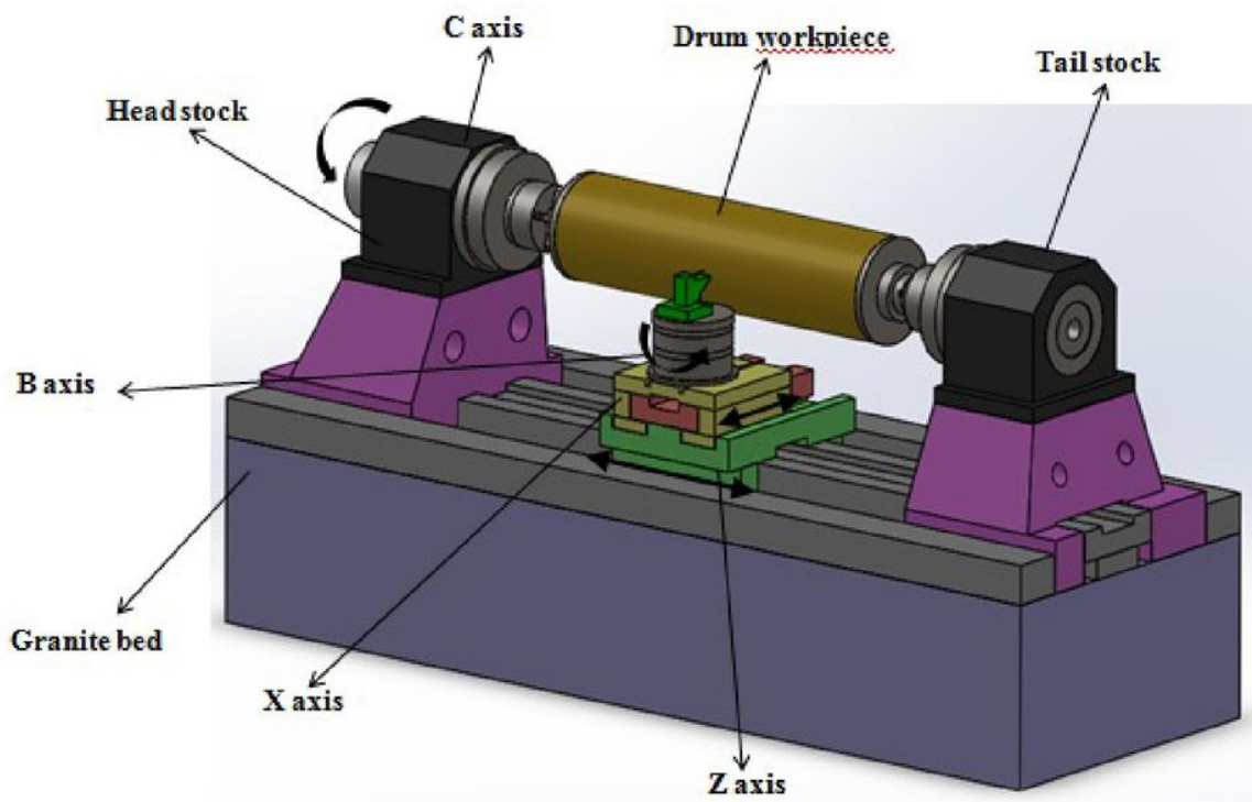
Figure 1: Structural layout of four-axis ultra-precision drum lathe
