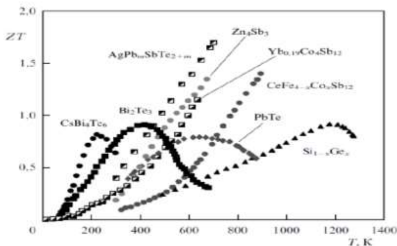
1-rasm. Istiqbolli materiallar ZT=\phi(T) bog'lanishi.
